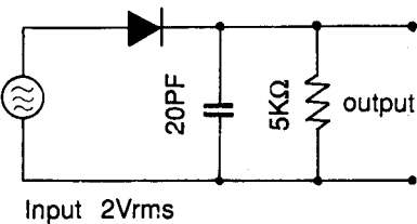
Rectification Efficiency Measurement Circuit
